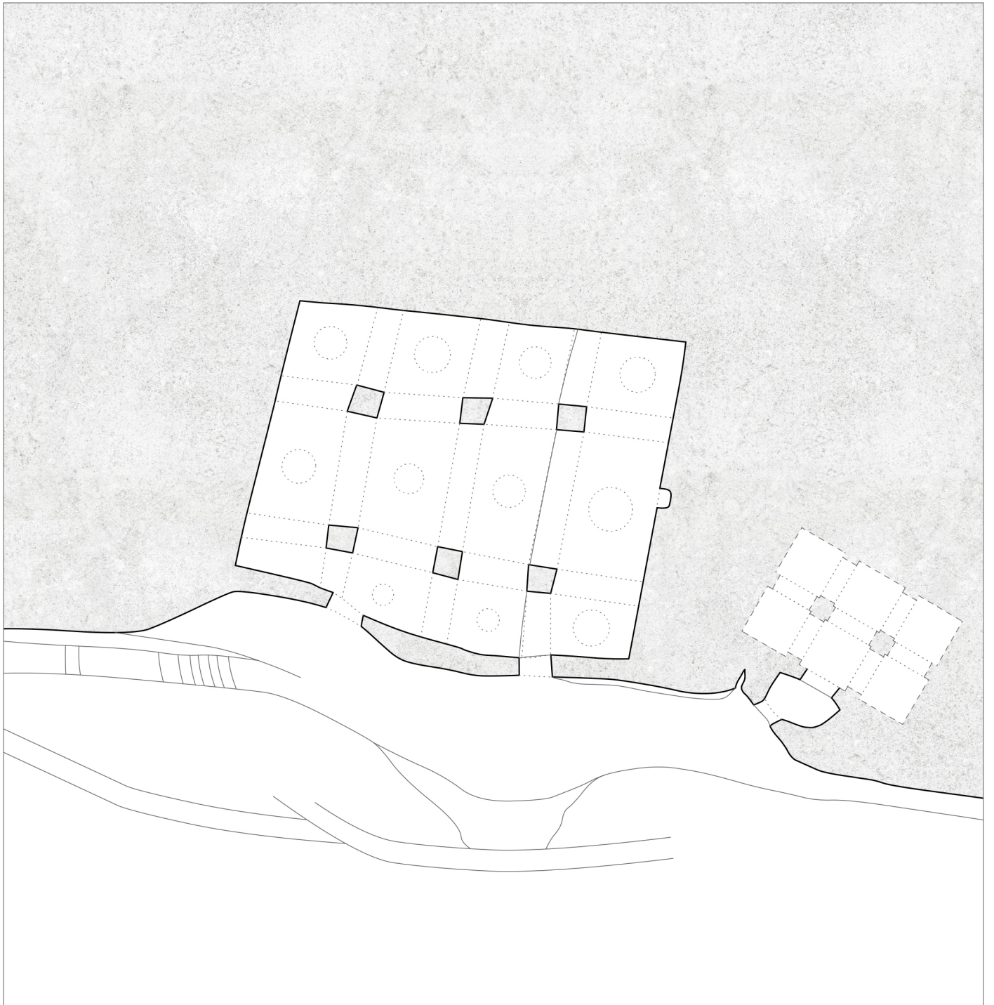
Medhane Alem Warq Amba Ground Floor Plan (2017)
